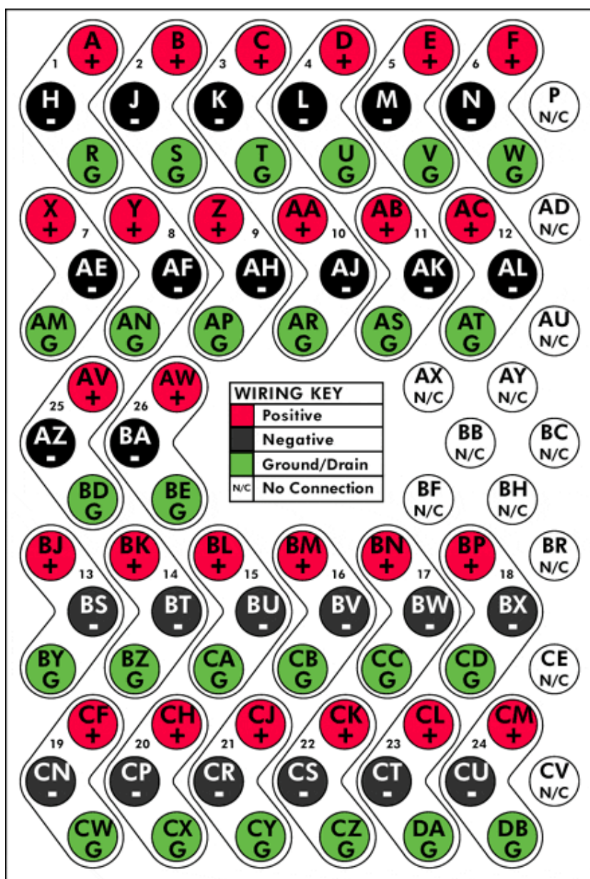
REAR VIEW OF MALE ELCO 90 PIN CONNECTOR FOR ADC PRO-PATCH
