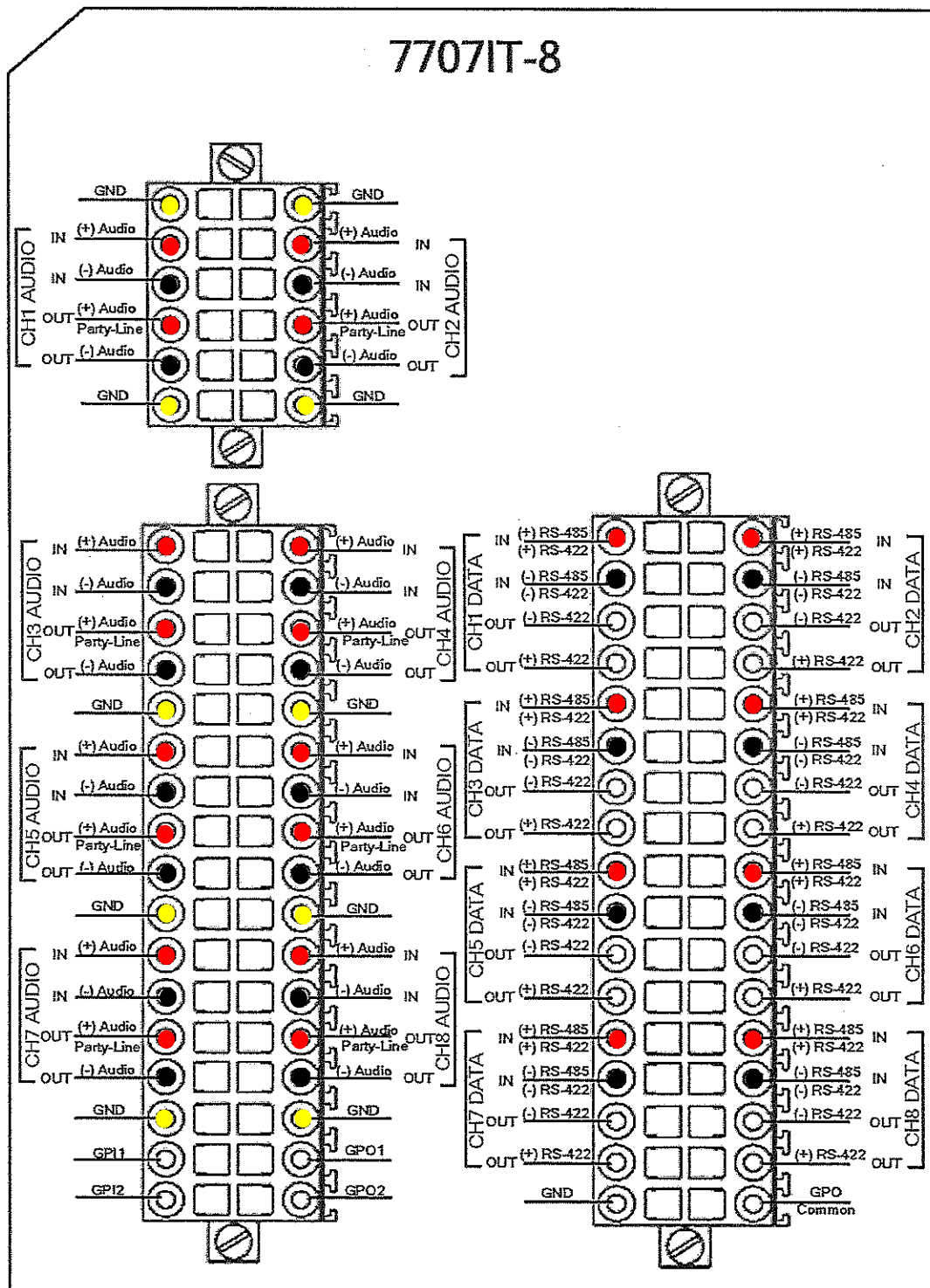
Figure 2-4: 7707IT-8 Terminal Block Signal Connections
