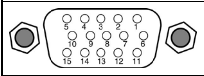
Figure A-2 LTC/GPI 15-Pin, Female, D-Sub Connector
