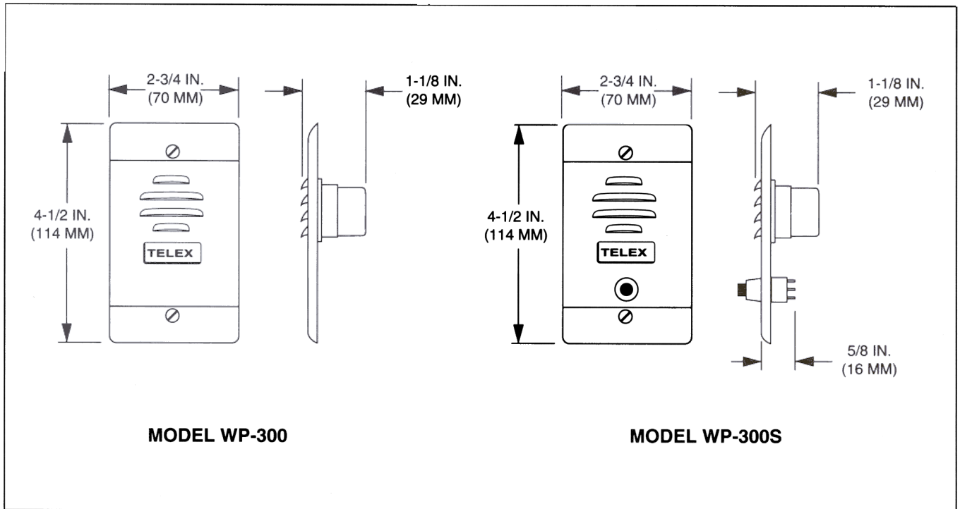
Dimension Drawings
