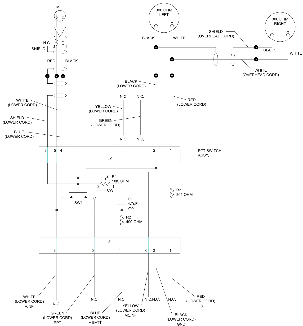
WIRING DIAGRAM
