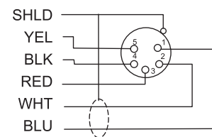
5 Pin Female
