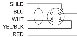
4 Pin Male
