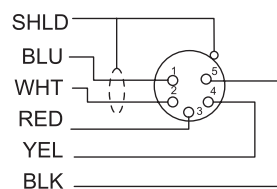
5 Pin Male
