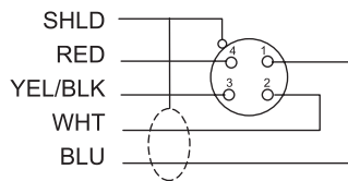
4 Pin Female
