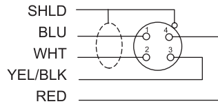
4 Pin Male
