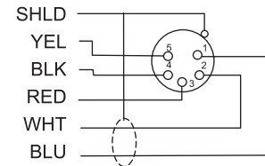
5 Pin Female
