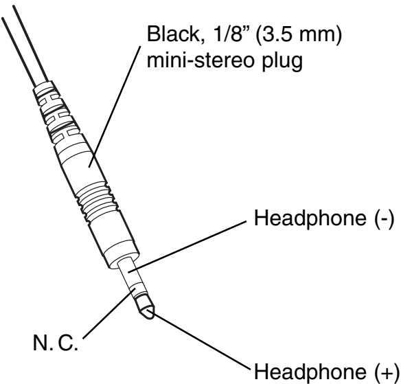
Headphone Connector
