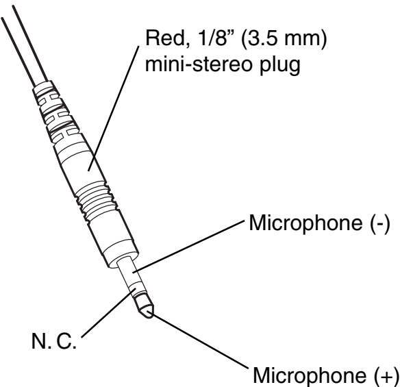
Microphone Connector
