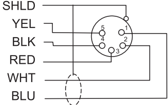
5 Pin Female
