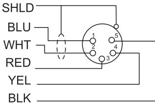
5 Pin Male
