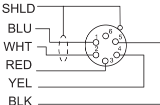
6 Pin Male
