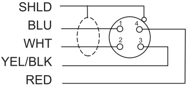
4 Pin Male
