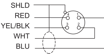
4 Pin Female
