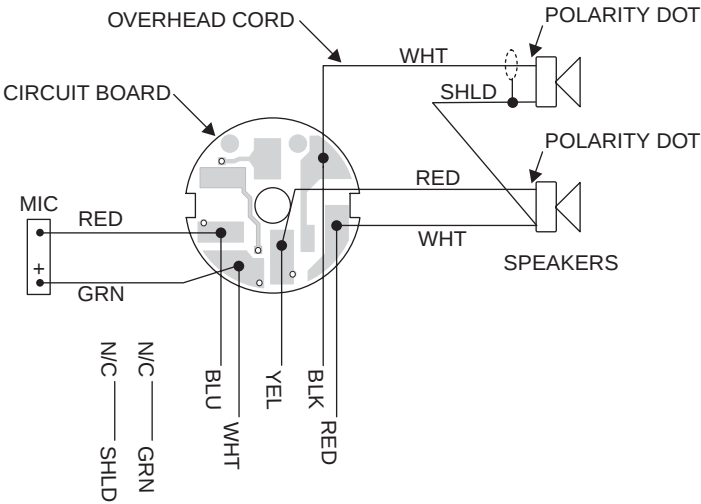
PH-44 Wiring Diagram
