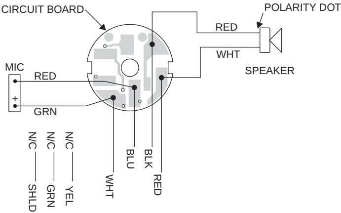
PH-88 Wiring Diagram
