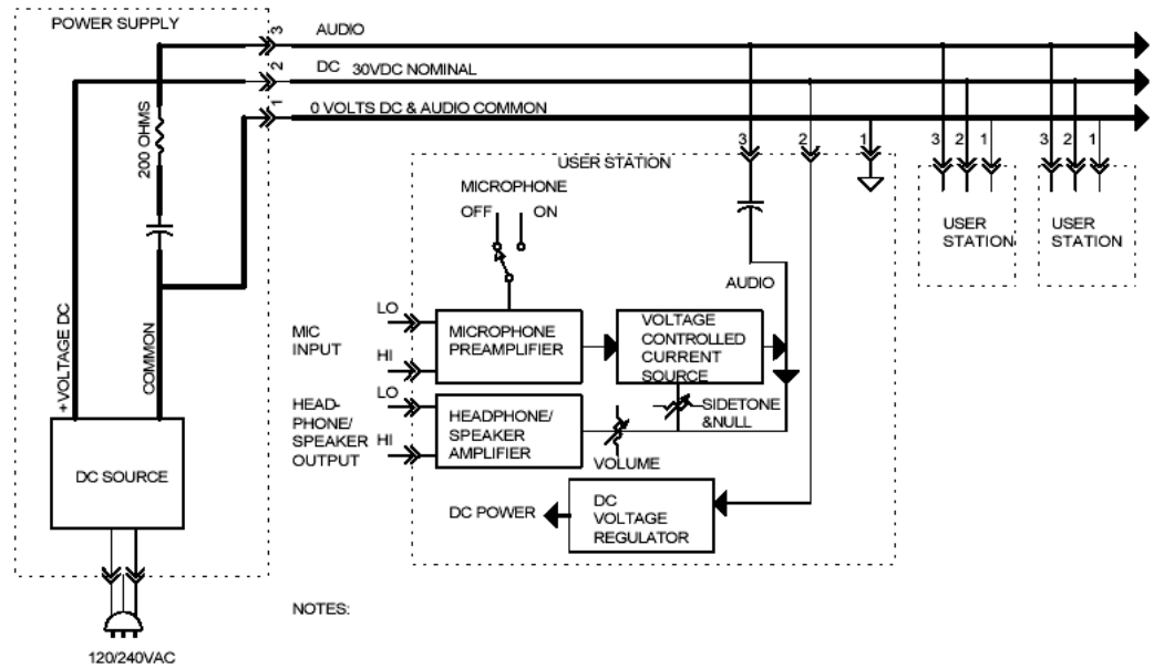
Figure 2.3 RTS™ TW intercom concept.
