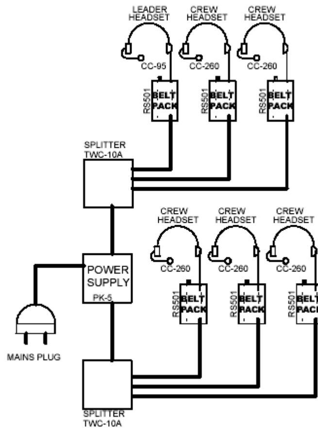
Figure 3.2 Generic single channel Clear-Com® system.
