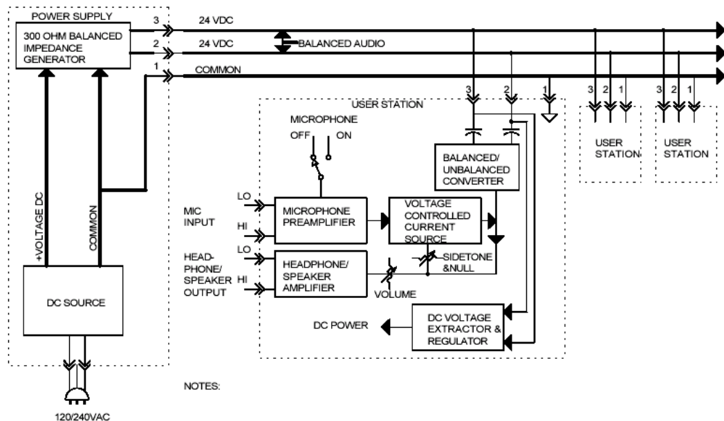
Figure 2.1 Audiocom® intercom concept.
