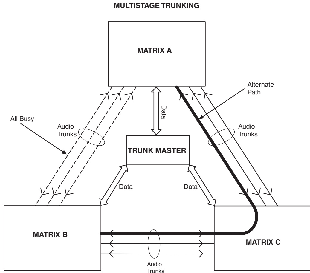
Figure 5.8 Multistage Trunking
