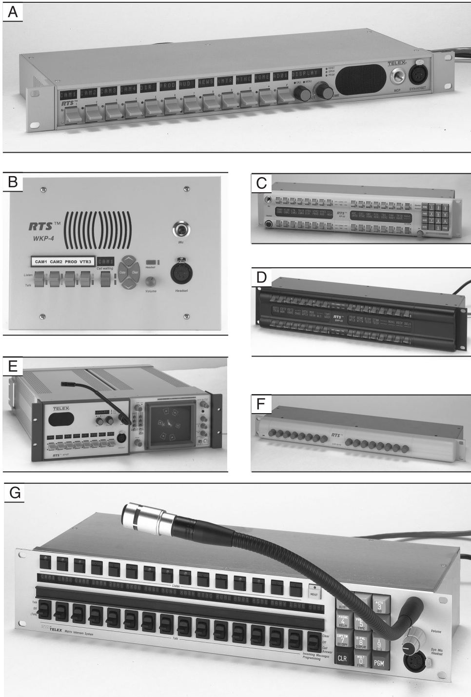
Figure 5.2 A wide variety of keypanel options exist. Here we have a selection of RTS™ keypanels that fit a wide range of needs. Small keypanels such as the (A) KP-12LK and (B) WKP-4 provide an interface for those with limited keypanel needs. The (G) KP-96-7, a medium sized unit, is the workhorse of the RTS™ keypanel line. The (C) KP-32 is the top of the line keypanel, and can be enhanced through additional options, such as the (D) EKP-32 expansion panel, and the (F) LCP-32/16 level control panel. The (E) KP-8T is an example of a specialty keypanel that makes use of an empty bay in a Tektronix vectorscope.
