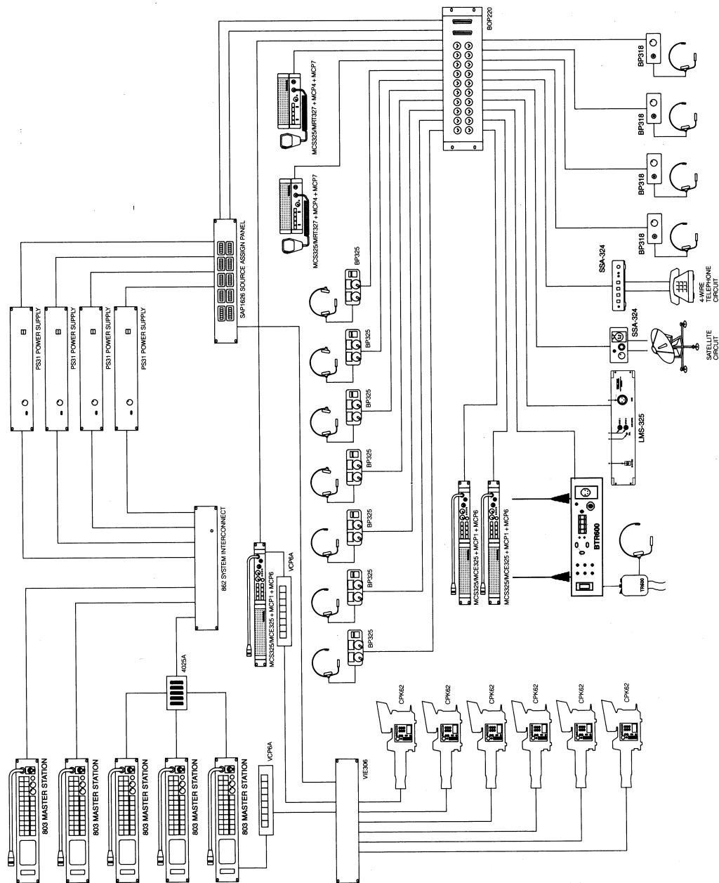
Figure 3.9 Large intercom system for television.
