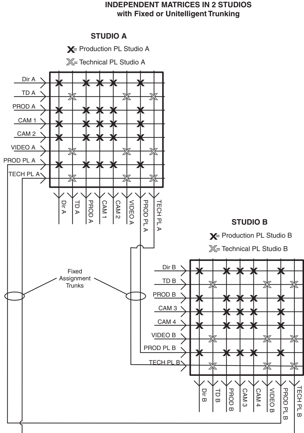
Figure 5.6 Fixed Trunking
