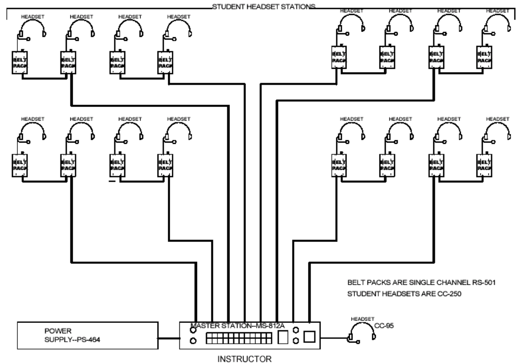
Figure 3.7 Clear-Com based training intercom system.
