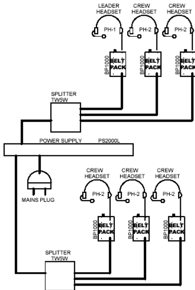
Figure 3.1 Generic single channel Audiocom® system.
