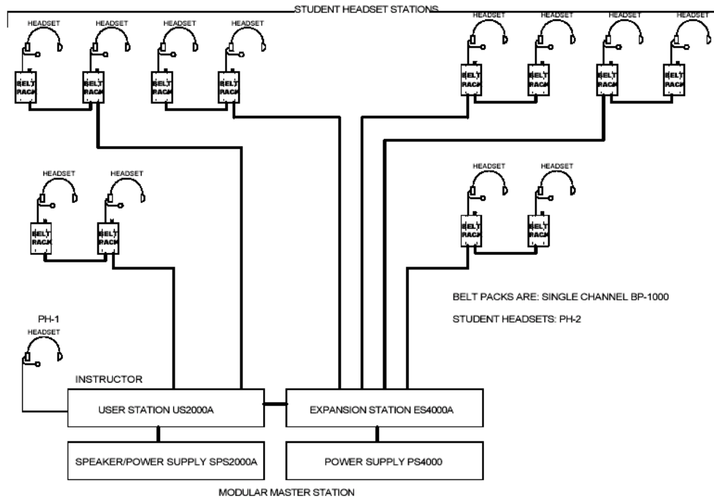
Figure 3.6 Audiocom based training intercom system.
