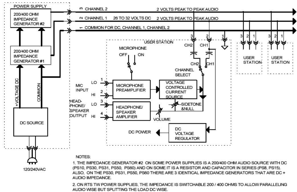
Figure 2.3 RTS™ TW intercom concept.
