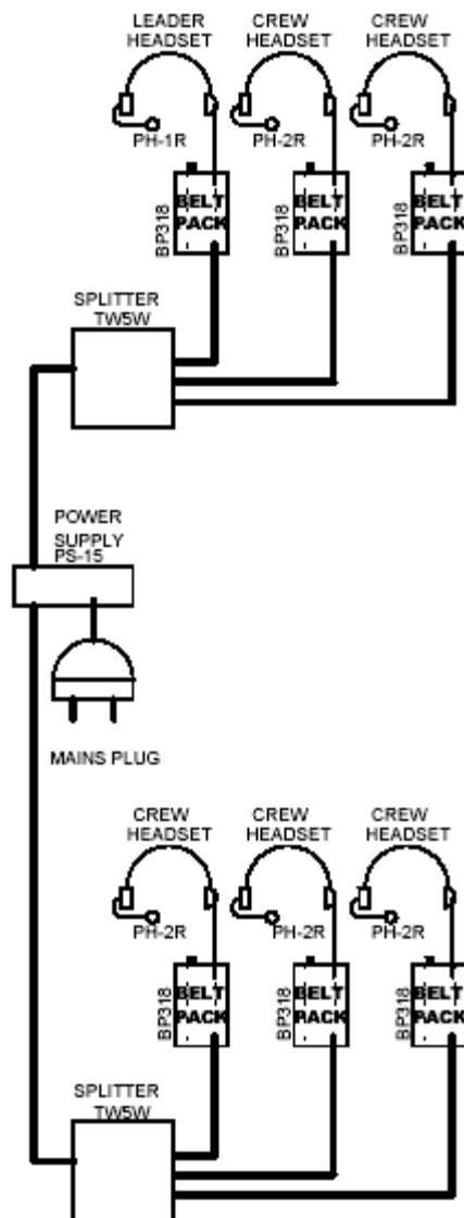
Figure 3.3 Generic single channel RTS™ TW system.
