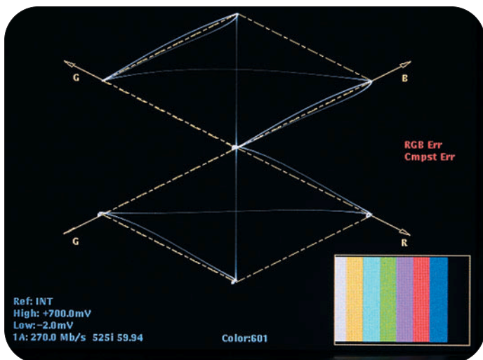
► Figure 14: P'b timing error shown on Diamond display
