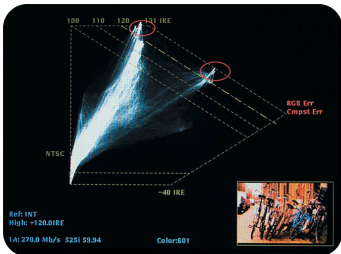
► Figure 26: Live video signal monitored with the Arrowhead display showing clear indication of a composite gamut error
