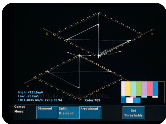
► Figure 12: Split Diamond display using SMPTE Color Bars
