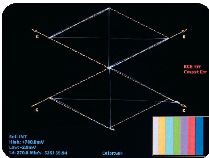
► Figure 7: 100% Color Bars with red error
