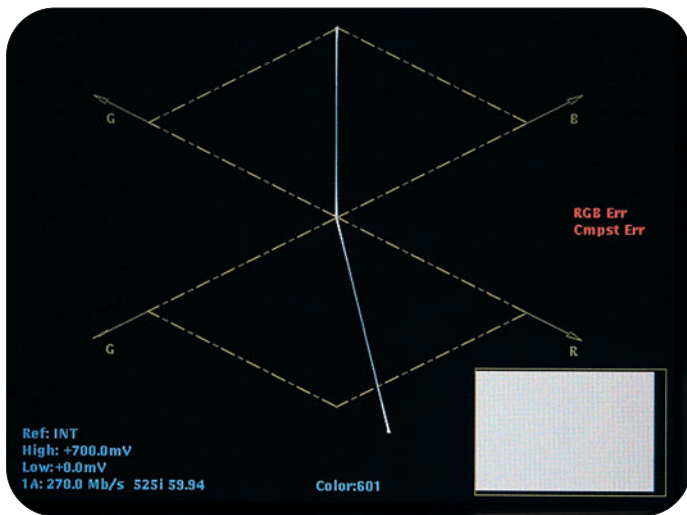
► Figure 21: Red gain error on Diamond display
