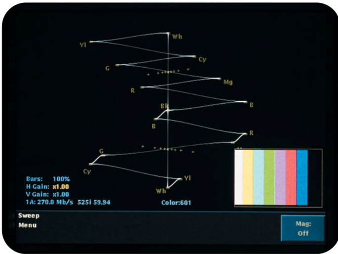
► Figure 28: Lightning display with Color Bars signal
