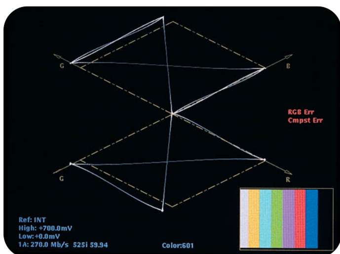
► Figure 6: Diamond display using 100% color bars with green amplitude error
