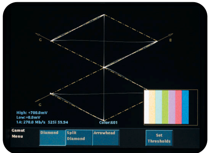
► Figure 2: Diamond display with 100% Color Bars
