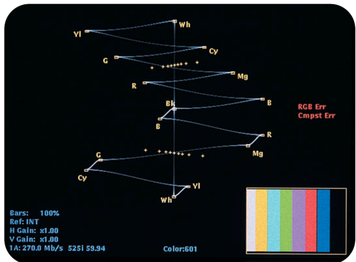
► Figure 32: P'b delayed timing error on Lightning display
