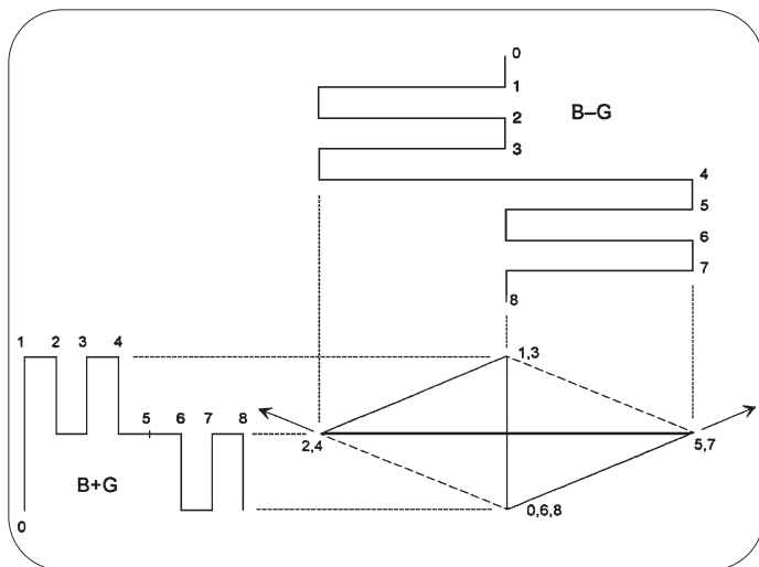
► Figure 4: Formation of upper diamond with G' and B'
