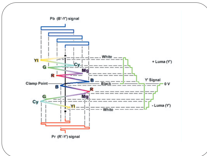
► Figure 27: Construction of Lightning display
