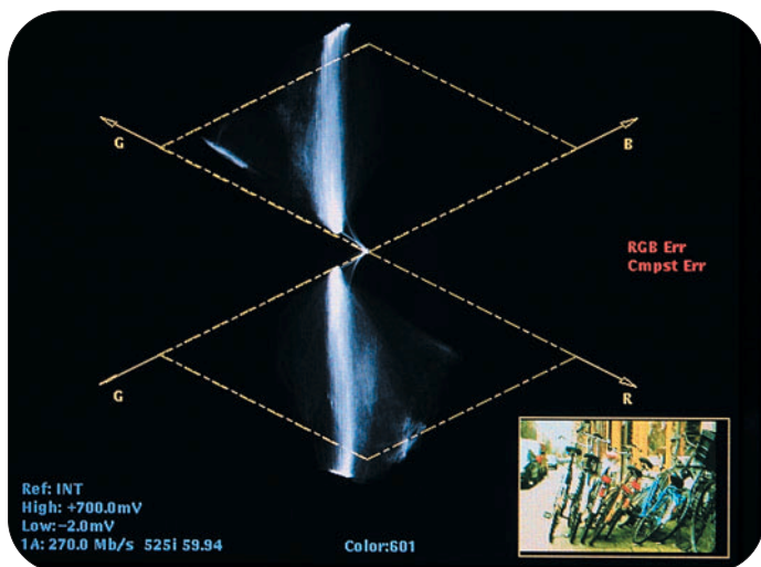
► Figure 18: Live signal with green balance error
