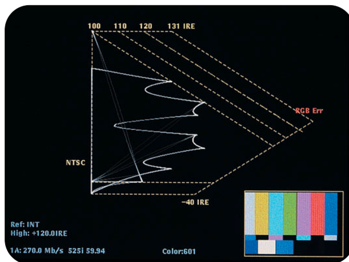
► Figure 24: Arrowhead display showing SMPTE Color Bars
