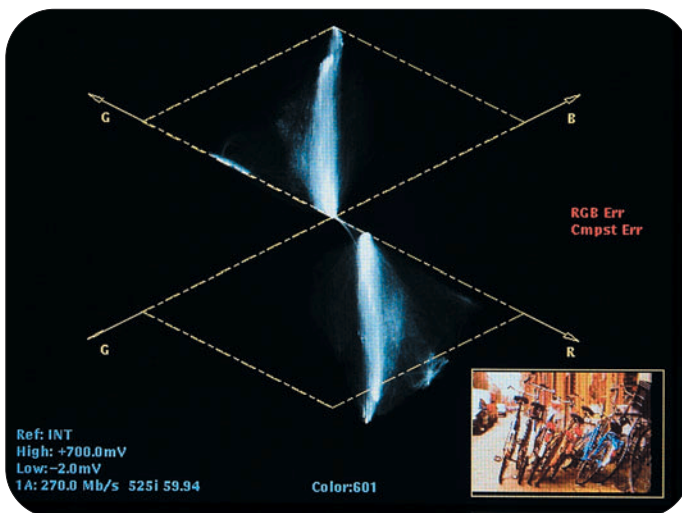
► Figure 16: Live signal with red balance error
