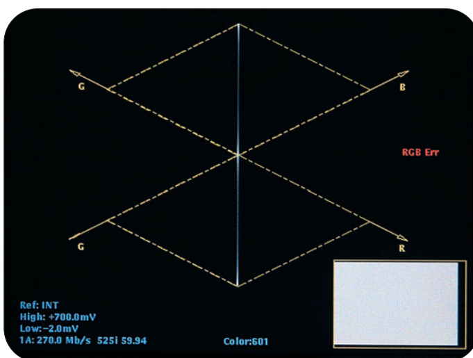
► Figure 19: Correctly balanced white field shown on Diamond display
