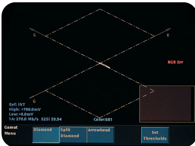
► Figure 15: Red balance error on Diamond display
