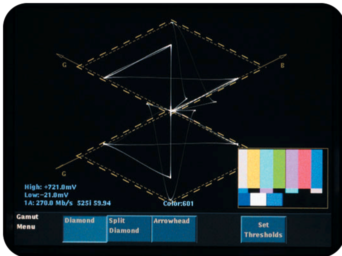
► Figure 9: Diamond display using SMPTE Color Bars signal exceeds R'G'B' limits
