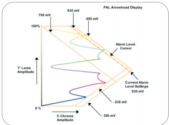
► Figure 22: PAL Arrowhead construction
