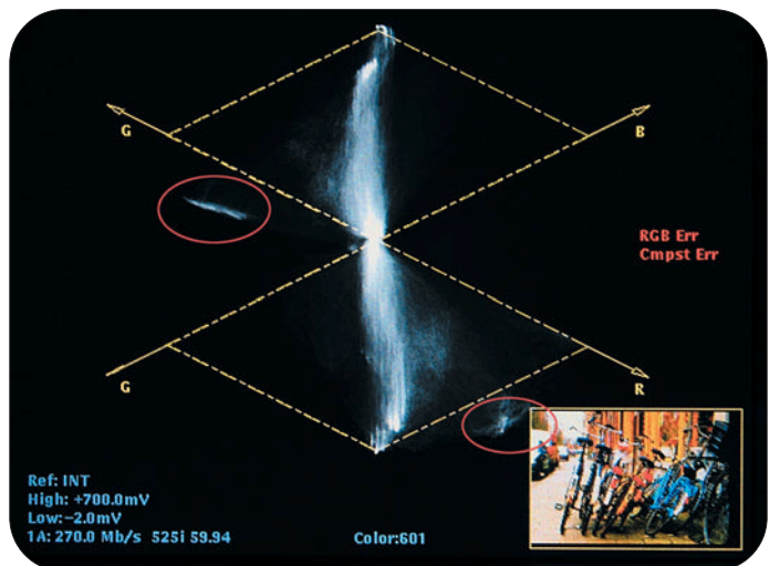
► Figure 11: Diamond display with live signal and gamut errors
