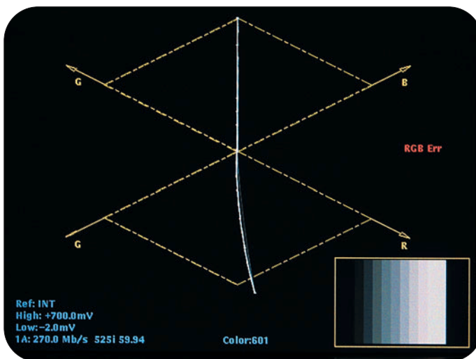
► Figure 8: 10 step staircase with red imbalance
