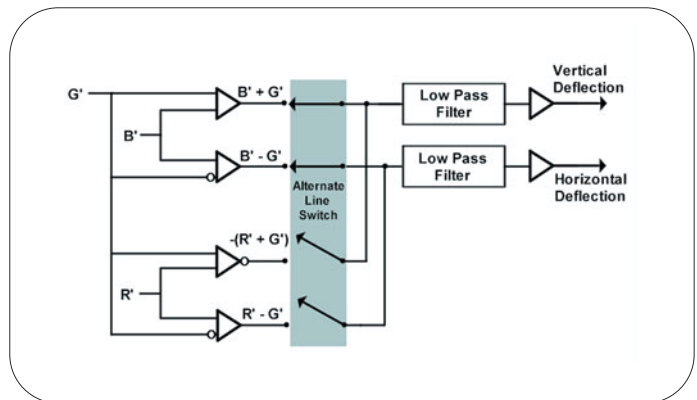
► Figure 5: Low pass filter reduces high frequency transients that exceed gamut limits
