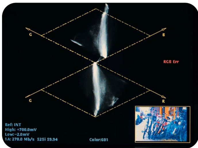
► Figure 17: Live signal with blue balance error
