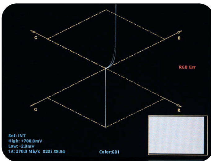
► Figure 20: Blue gamma error on Diamond display
