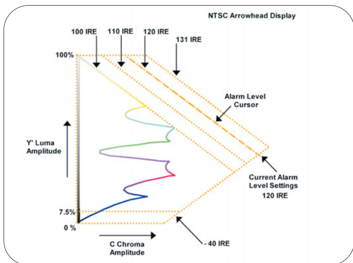
► Figure 23: NTSC Arrowhead construction
