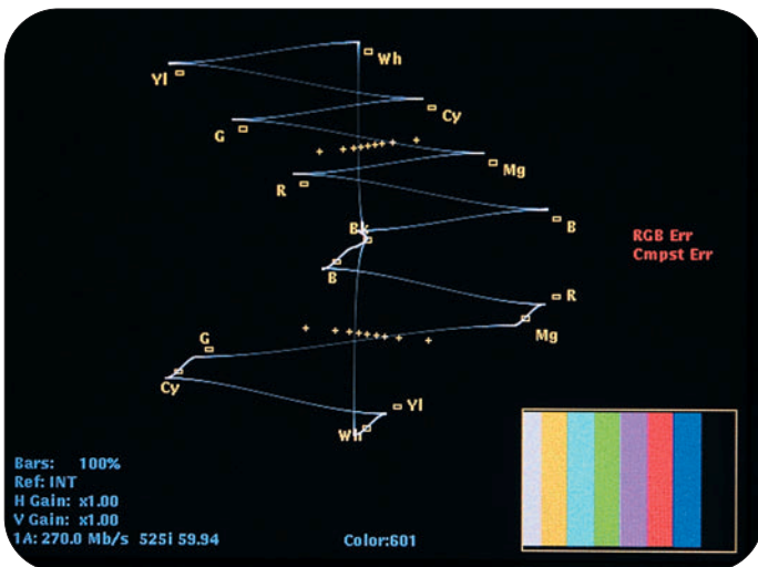
► Figure 29: Luma gain error on Lightning display
