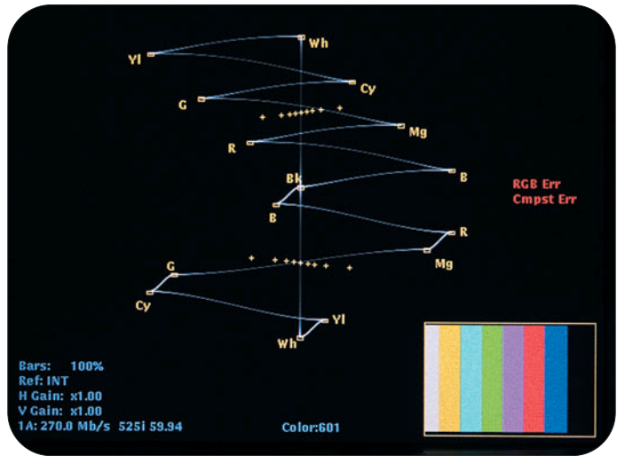
► Figure 31: P'b advanced timing error on Lightning display
