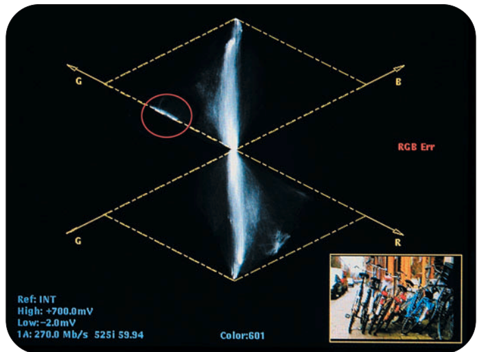
► Figure 10: Diamond display with live signal
