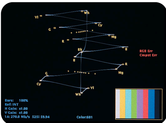
► Figure 30: P'b gain error on Lightning display
