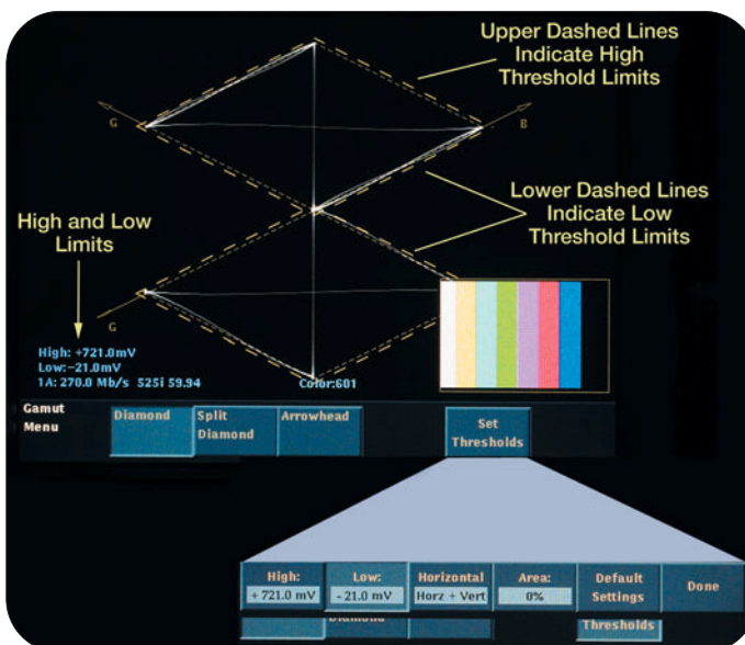
► Figure 13: Selection of user limits on WFM700
