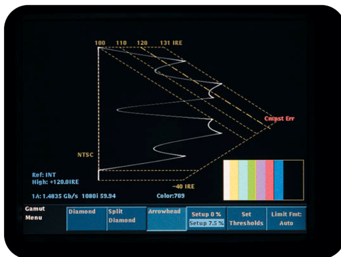
► Figure 25: Arrowhead display with 100% Color Bars Signal
