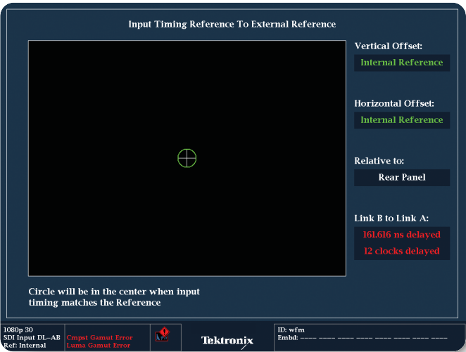
► Figure 16. Inter-channel Timing measurement of a Dual Link signal.
