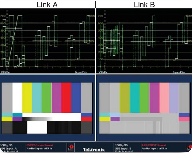
► Figure 9 Waveform displays of Dual Link A and B signals for Y'C'bC'r 4:4:4 12-bit format.
