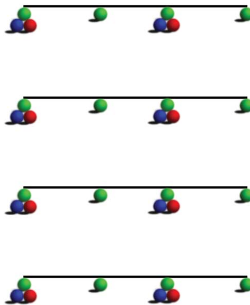
► Figure 1. 4:2:2 Sampling Structure.
