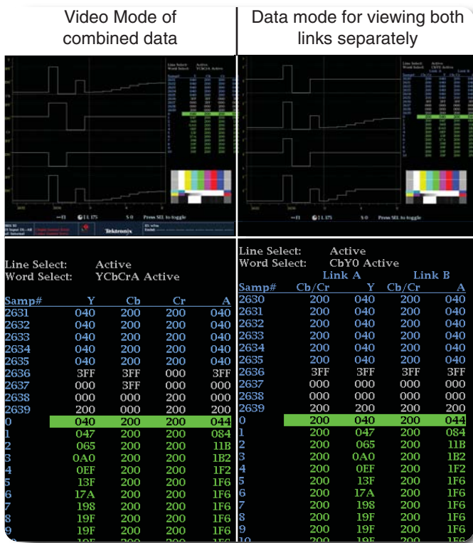
► Figure 5. Data mode views for combined and separate links.
