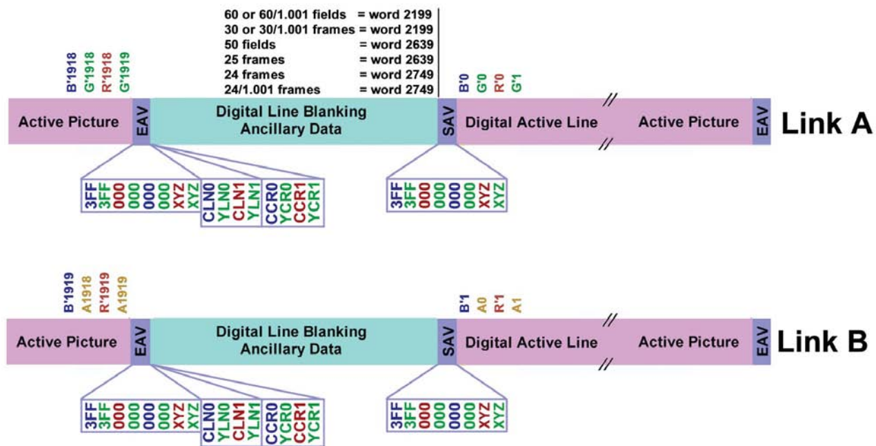
► Figure 6. Data Structure of R'G'B'(A) 4:4:4:4 format for both Link A and Link B.
