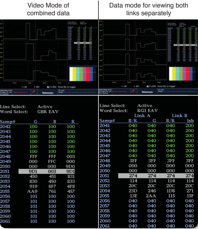
► Figure 18. EAV Data mode view of 2048x1080 R'G'B' 12-bit Dual Link format.
