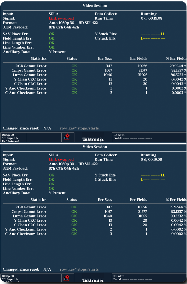
► Figure 11. Video Session displays of WFM7120 showing that the error messages for Links A and B.
