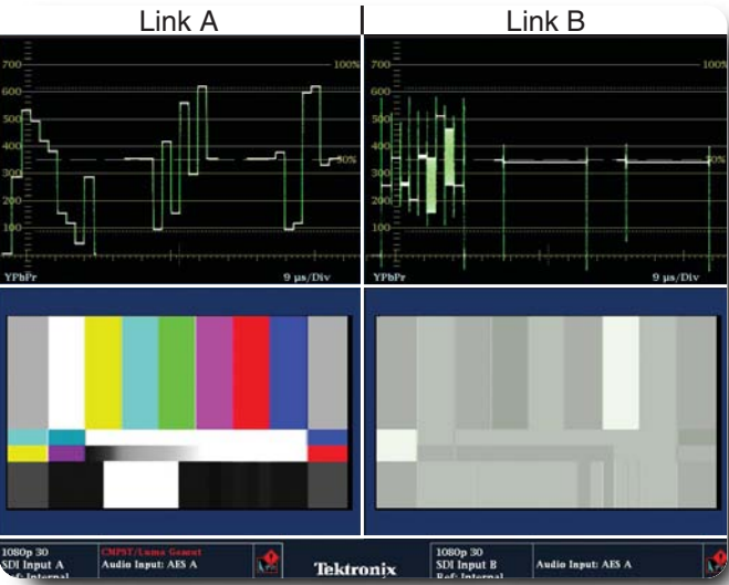
► Figure 10. Waveform displays of Dual Link A and B signals for Y'C'bC'r(A) 4:2:2:4 12-bit format.
