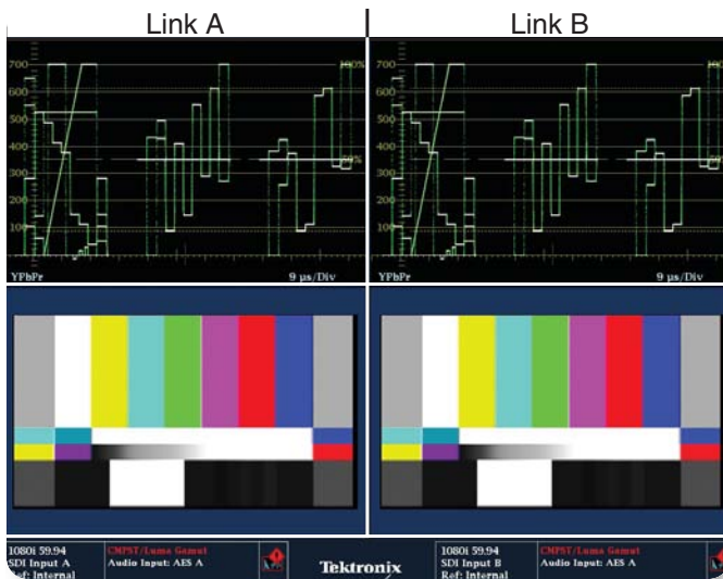
► Figure 2. Link A and Link B of a 4:2:2 10-bit 1920x1080 60p SMPTE219 color bar signal.
