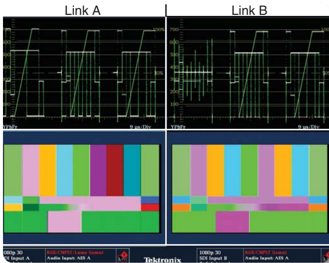
► Figure 7. Waveform displays of Dual Link A and B signals for R'G'B' 4:4:4 12-bit format.
