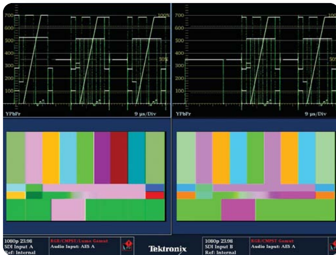
► Figure 3. Waveform displays of Dual Link A and B signal for R'G'B' (A) 4:4:4:4 format.
