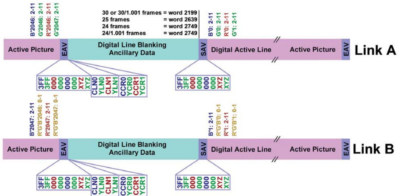
► Figure 17. 2048x1080 R'G'B' 12-bit Dual Link data structure format.
