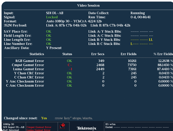
► Figure 14. Video Session Display showing SMPTE352M payload.
