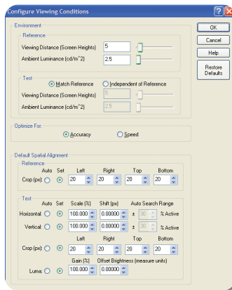
► Figure 16. Viewing Conditions Dialog.
