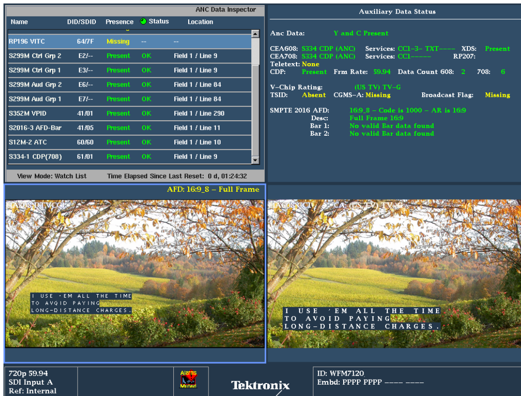
Figure 4. FlexVu™ showing simultaneous picture decodes of 608 and 708 closed captions
