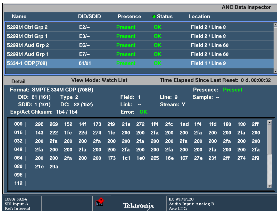
Figure 5. ANC Data Inspector display showing CEA 708 closed captions.
