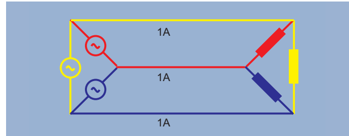
Figure 7. Delta connection - three-phase, three wires.
