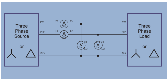
Figure 13. Three-phase, three-wire, 2 wattmeter method.
